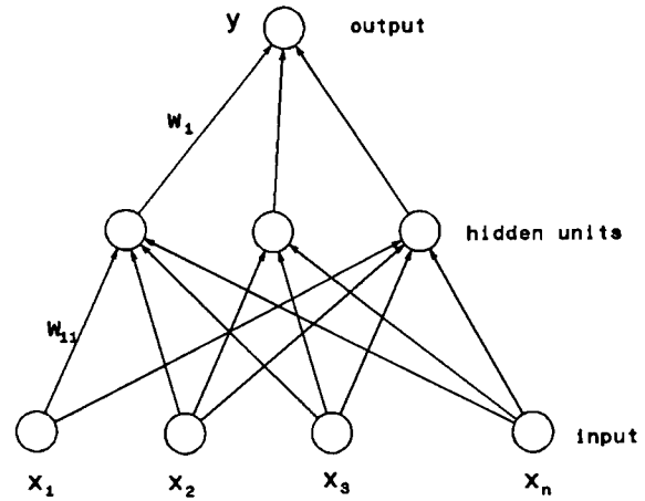
FIGURE 1. Single hidden layer feedforward neural net.
